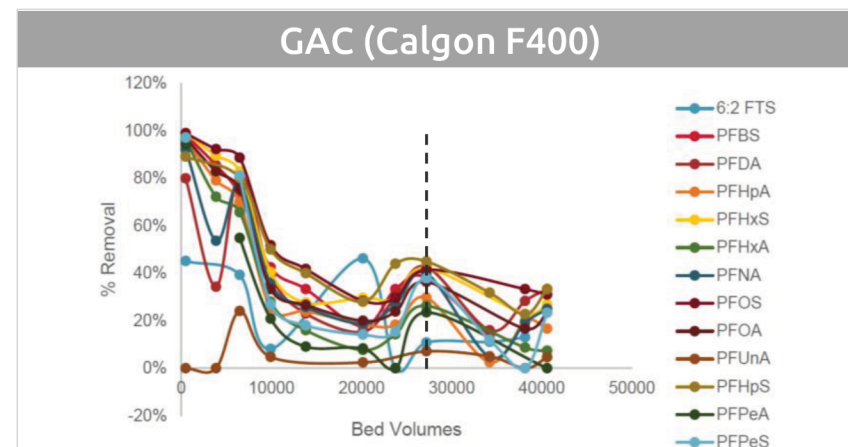
Figure 4-36. Concentrate Pilot Results – PFAS of Interest (Column 2 – Calgon, EBCT – 10 minutes)
