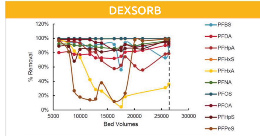
Figure 4-29. Concentrate Pilot Results – PFAS of Interest (Column 3 – NS)
